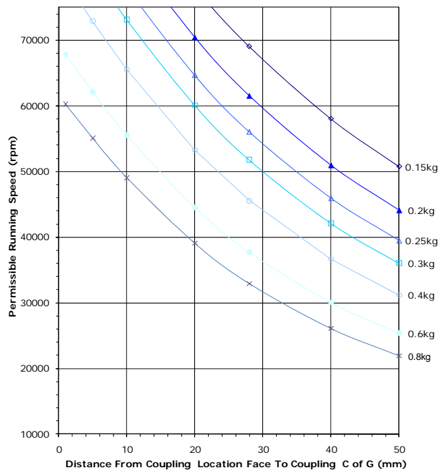
Permissible Speed vs Coupling C of G Overhang
